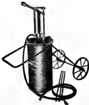
No. 3. A real whitewash sprayer powerful enough for tree spraying.
